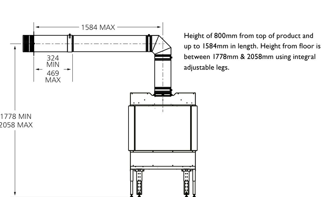
Horizontal balanced flue installation
