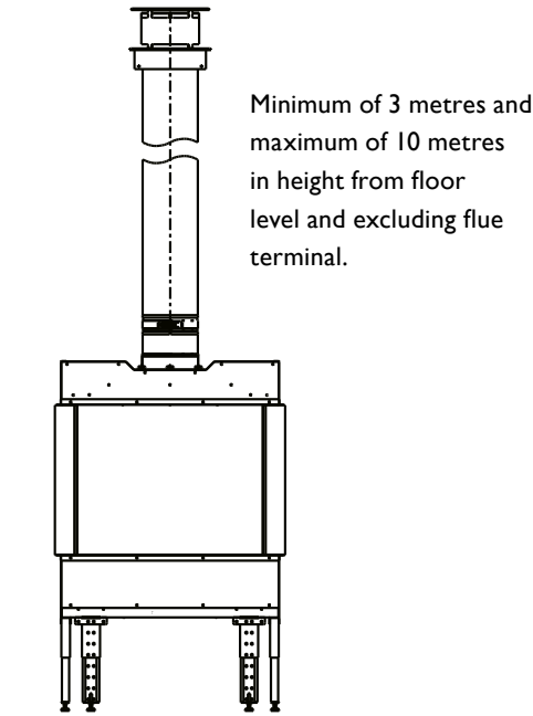
Vertical balanced flue installation
