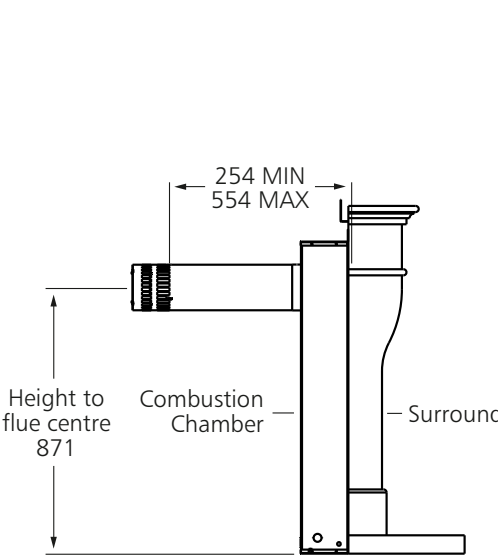
Horizontal balanced flue Installation
