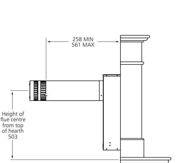
Horizontal balanced flue installation
