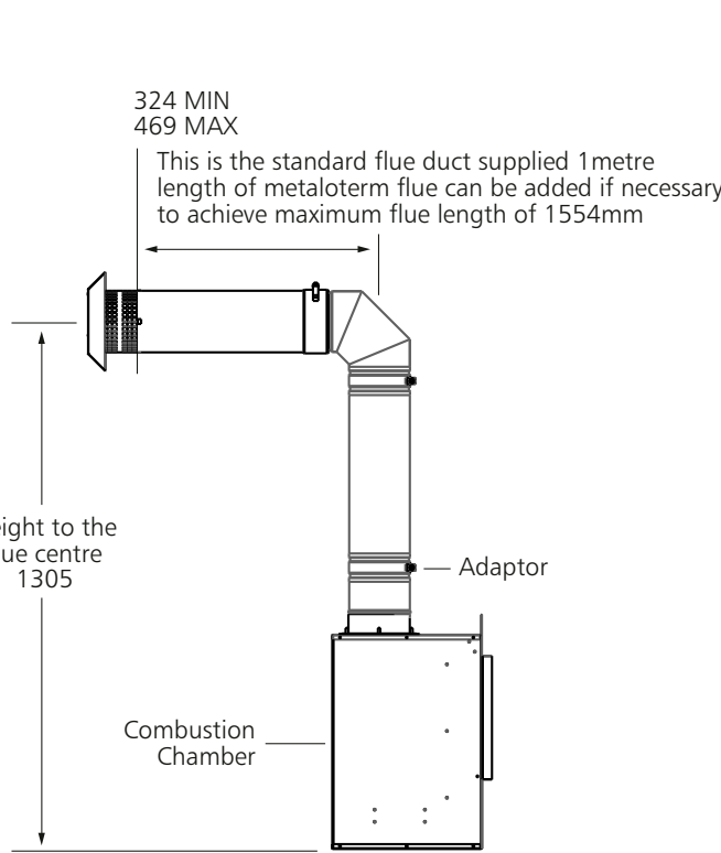
Horizontal balanced flue installation
