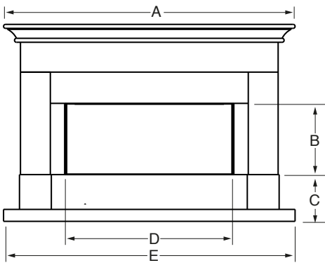
Front view 58L
