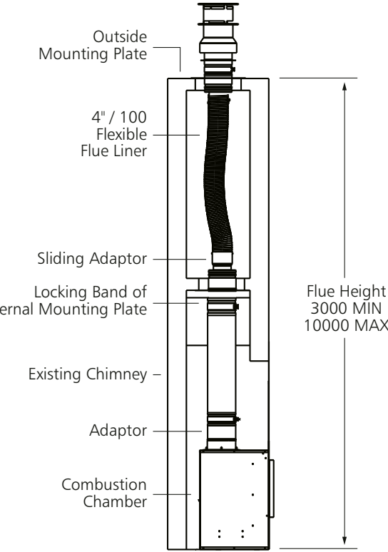
Chimney conversion balanced flue kit
