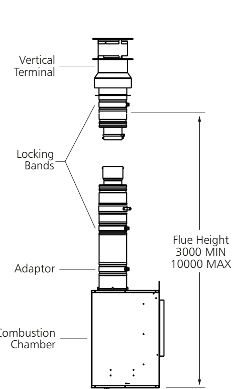
Vertical balanced flue installation
