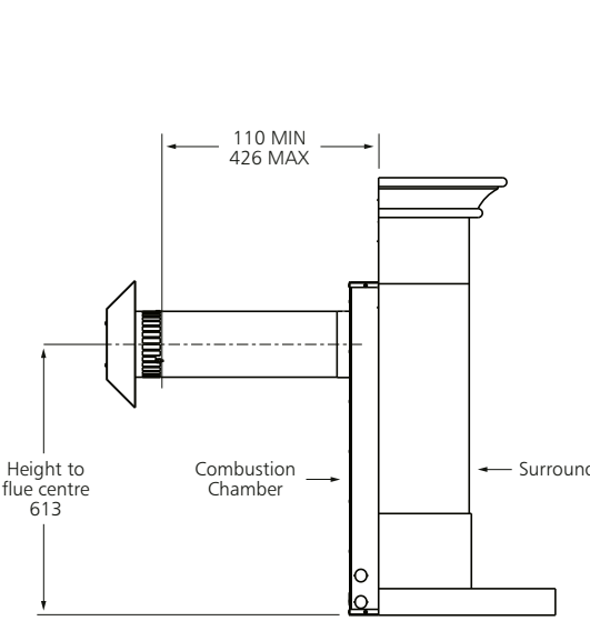
Chimney conversion balanced flue kit
