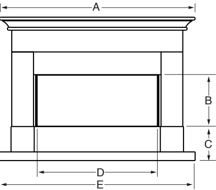
Front view 54L
