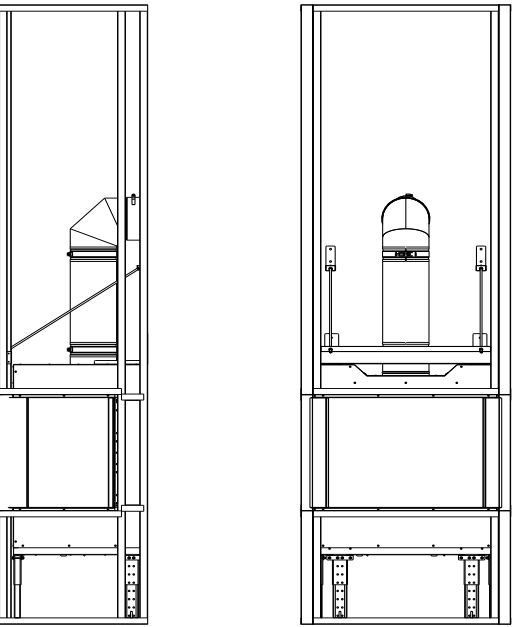
FALSE CHIMNEY STUDWORK
