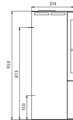
WESTFIRE.UNIQ.46 (FORMERLY UNIQ 18 WITH LOGDOOR) WEIGHT: 90 KG
