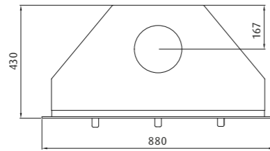
WESTFIRE.UNIQ.35 / INSERT 4-SIDED FRAME WEIGHT: 75 KG
