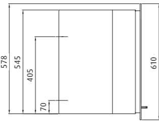
WESTFIRE.UNIQ.32 / INSERT NARROW 4-SIDED FRAME WEIGHT: 110 KG
