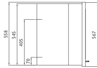
WESTFIRE.UNIQ.32 / INSERT WIDE 4-SIDED FRAME WEIGHT: 110 KG
