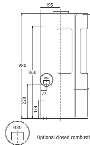
WESTFIRE.UNIQ.36 WESTFIRE.UNIQ.37 WEIGHT: 90 KG
