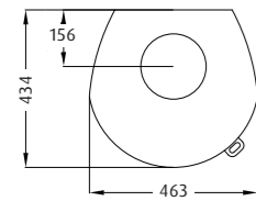
WESTFIRE.UNIQ.35 / 50 MM BLOCK WEIGHT: 95 KG
