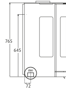
WESTFIRE.UNIQ.36 WESTFIRE.UNIQ.37 WALL-MOUNTED / WEIGHT: 85 KG
