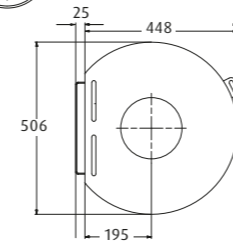
WESTFIRE.UNIQ.44 (FORMERLY UNIQ 17) WEIGHT: 82 KG
