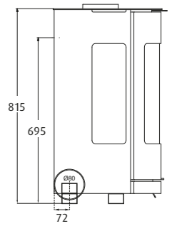
WESTFIRE.UNIQ.36 WESTFIRE.UNIQ.37 COMPACT / WEIGHT: 85 KG
